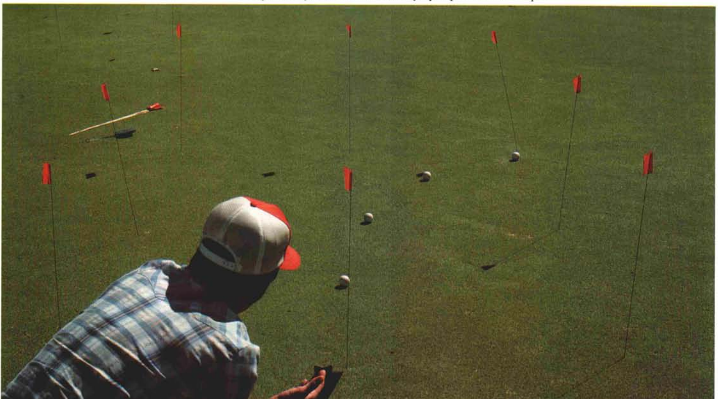
Figure 3. Checking stimpmeter speed by rolling crossways across a slope (shown here) distorts readings, whether you're using the formula or the traditional forward-reverse averaging method of calculation. When using the formula to compute green speed on a slope, always roll the ball directly upslope and downslope.
